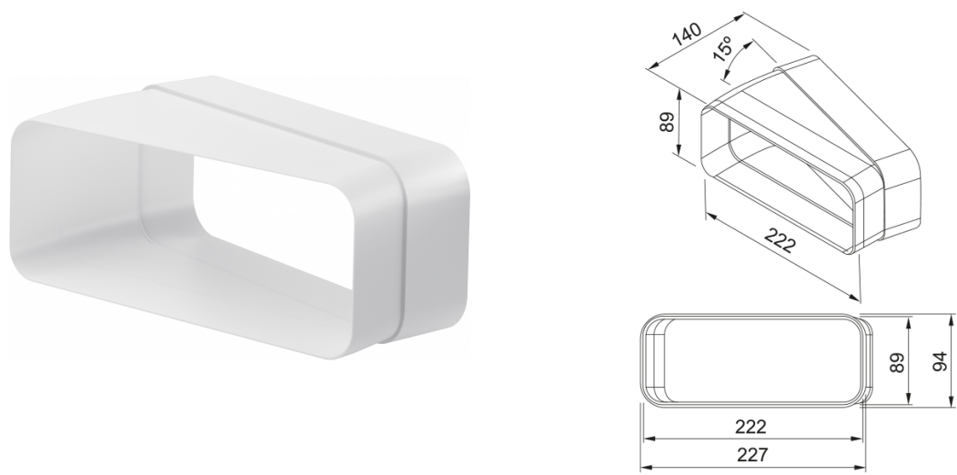
Coude horizontal F-RBH 150 15° long 140 mm Larg 227 mm Haut 94 mm
