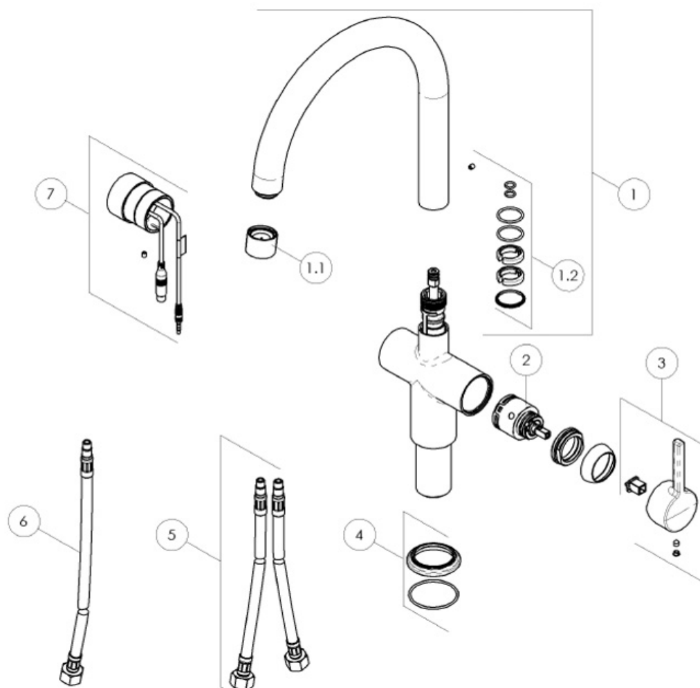
MFT Electronic J shape swivel, CHR
