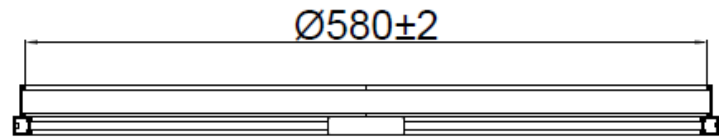
FRONT VIEW
