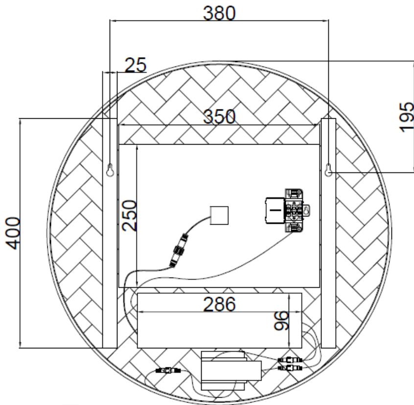
BACK VIEW
