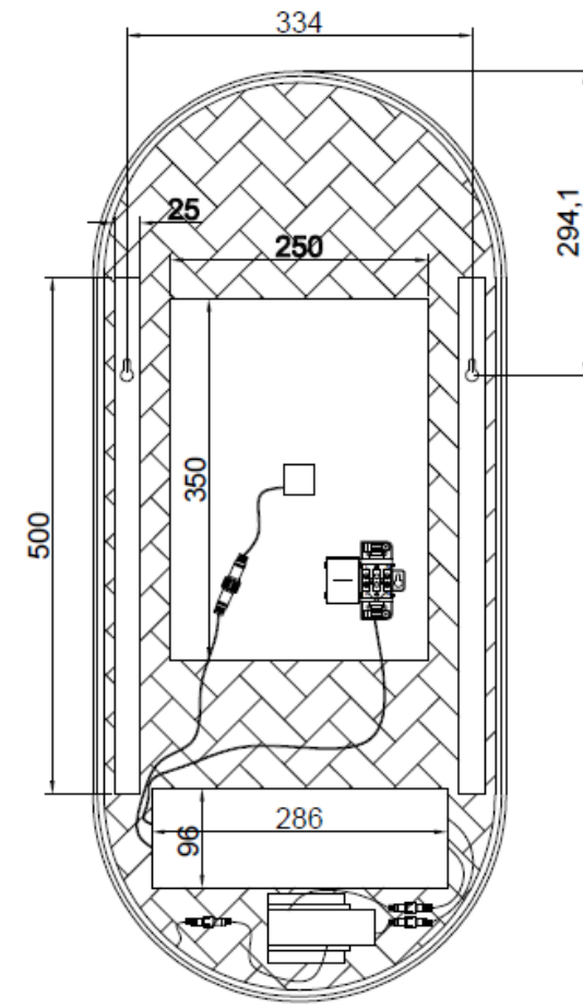
BACK VIEW
